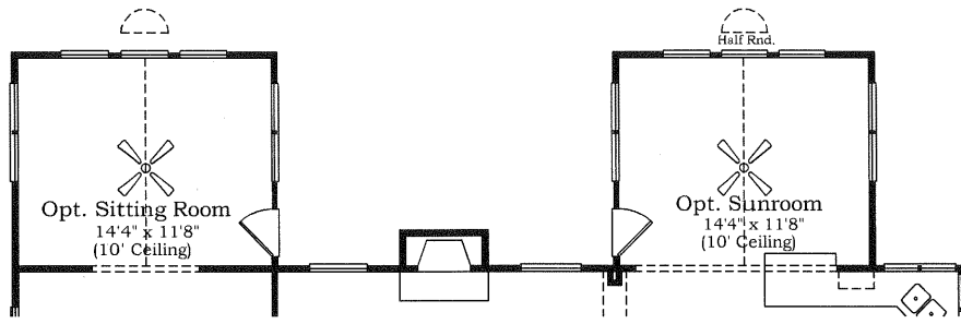
Partial First Level Plan w/ Opt. Sitting Room and Opt. Sunroom
