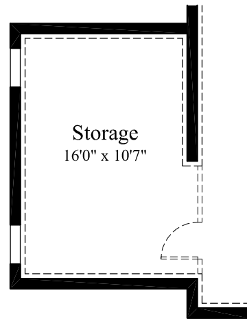
Partial Basement Plan w/ Optional Side Sunroom
