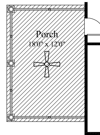
Partial First Floor Plan w/ Optional Porch
