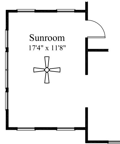
Partial First Floor Plan w/ Optional Side Sunroom
