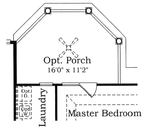
Partial Plan w/ Opt. Covered Porch Above Opt. Sunroom
