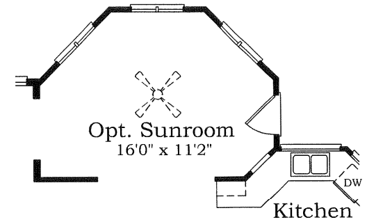
Partial Plan w/ Opt. Sunroom
