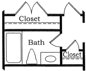
Partial Plan w/ Opt. Full Bath
